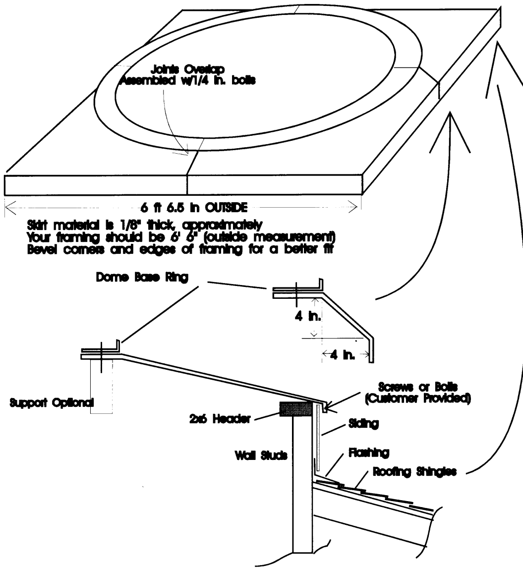
Typical Installation
